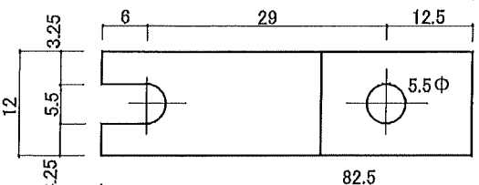
1PA-2 (1PA-2K)
